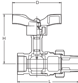
Dimensions of CTLTU
