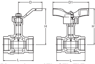
Dimensions of TL, CTL, TLT
