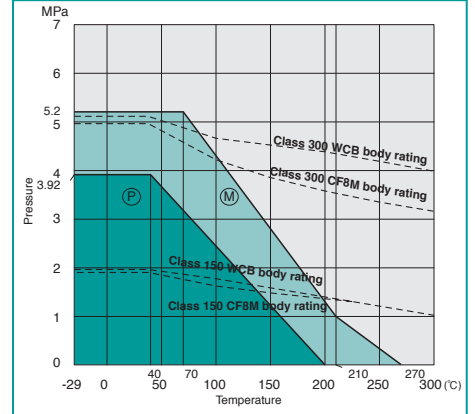
150/300UTAZ(M)/SCTAZM : NPS 4, 6
