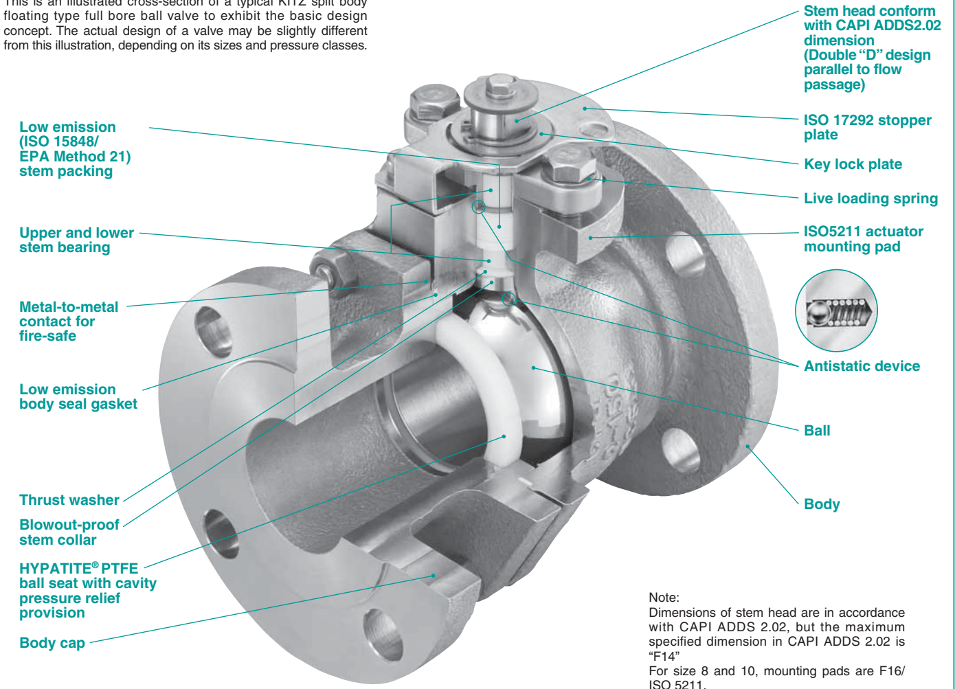
150UTDZ Size 2
