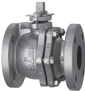
Blowout-proof stem
