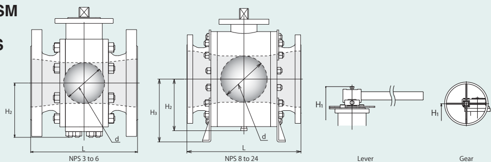
Dimensions of T60S/(G)-600UF3TCRSM, T60S/(G)-600SF3TCRS
