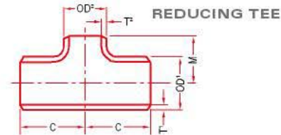
REDUCING TEE
