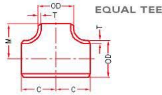
EQUAL TEE
